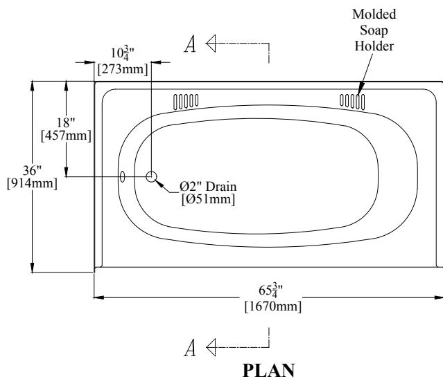
65 3/4" [1670mm] Bathtub w/ Molded Soap Holders & Removable Access Panel
